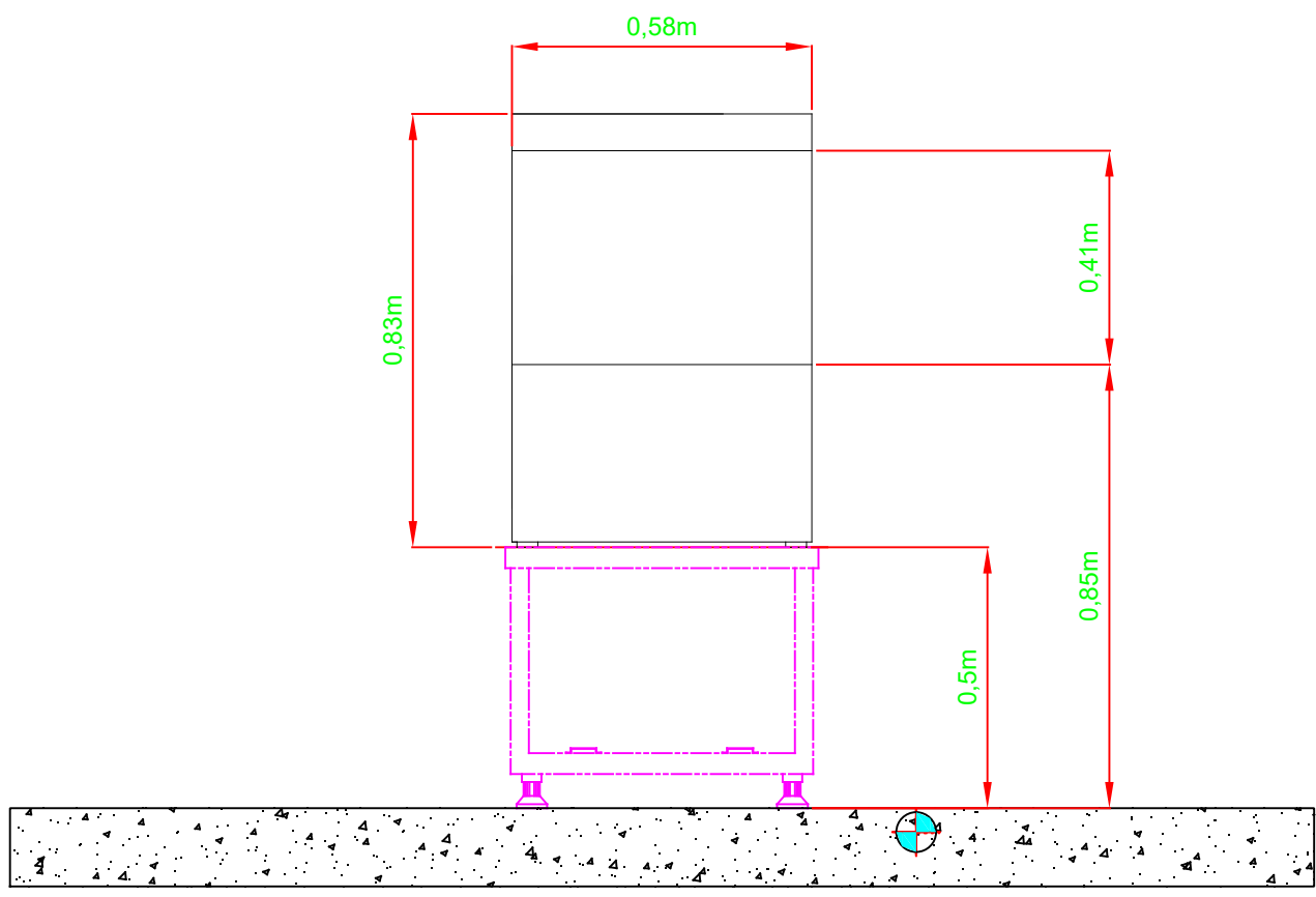
VISTA FRONTAL
